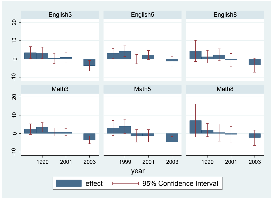
Figure 2: Event Study Estimates of the Impact of Sniper Attacks on Pass Rates
